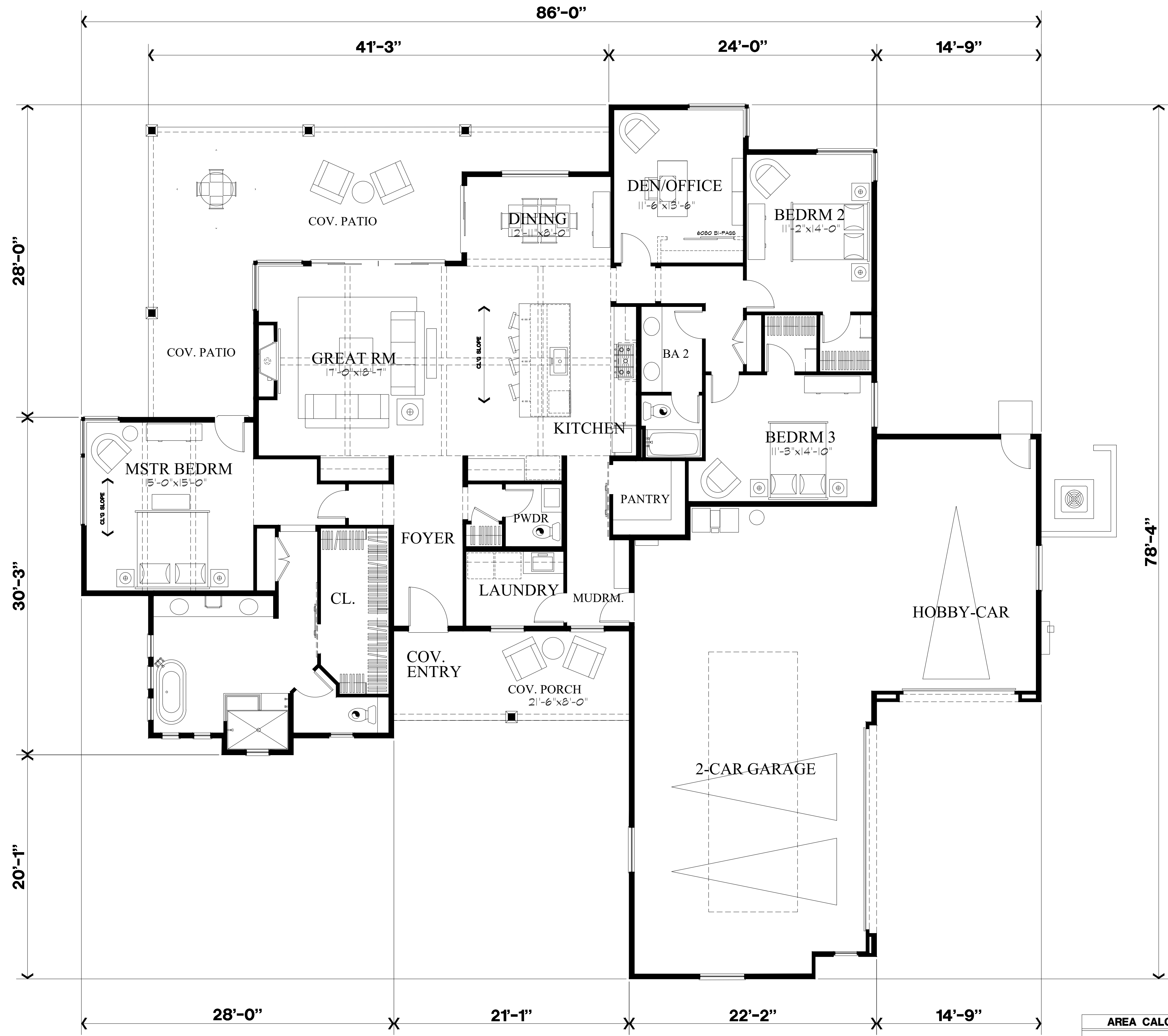
FLOOR PLAN
